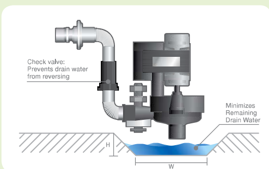
ONE-WAY FLOW
